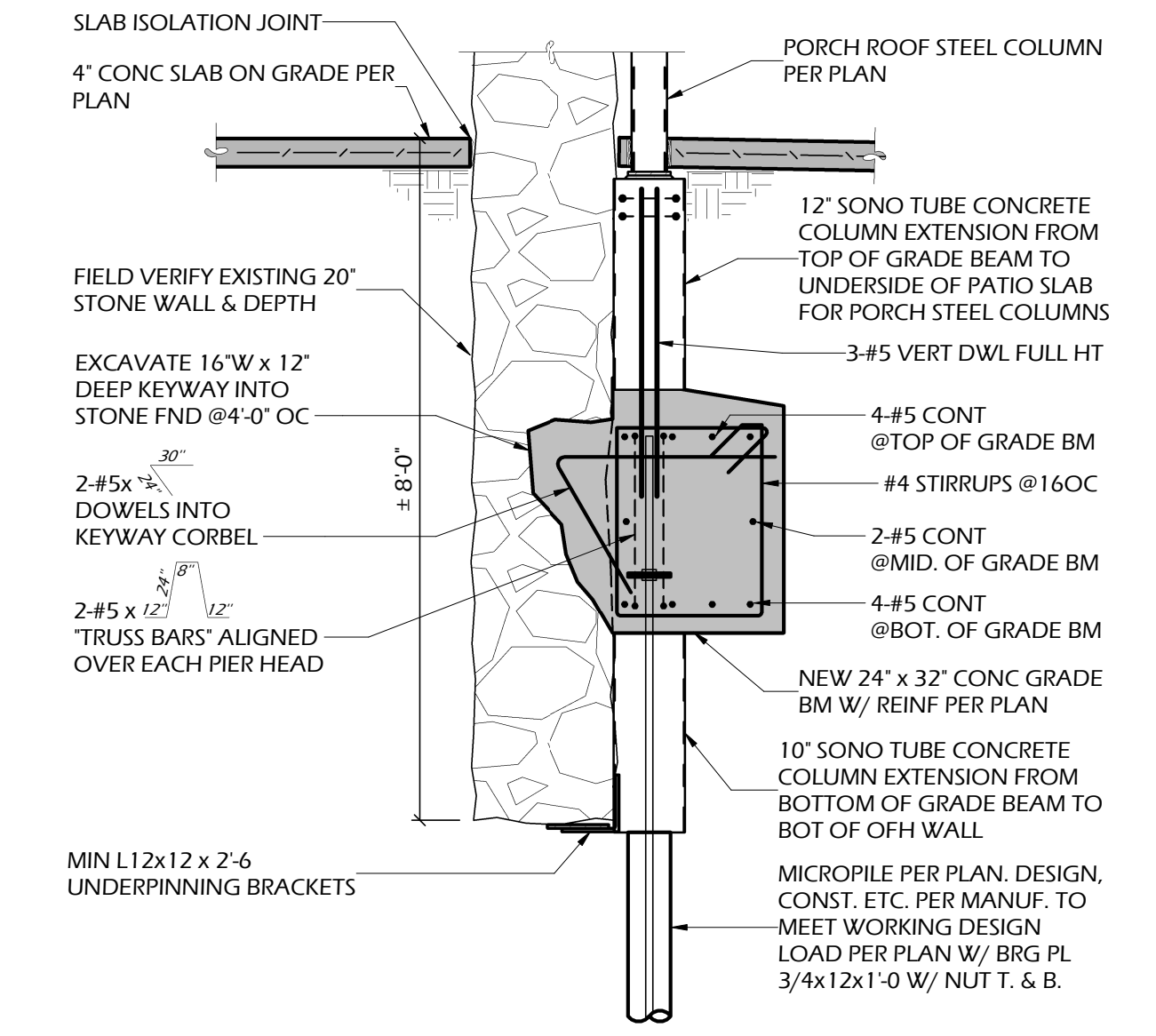
1 SECTION S3.10 1/2' = 1'-0"
