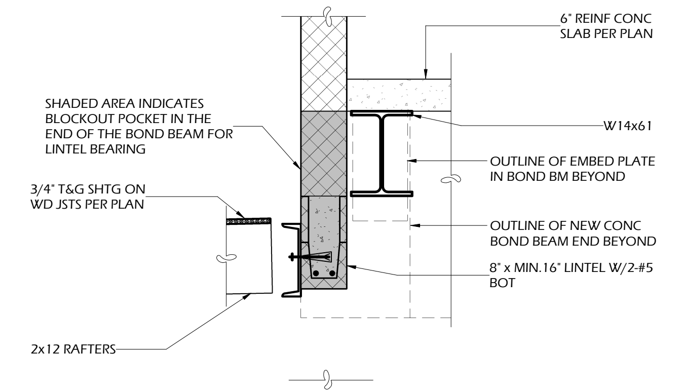
5 SECTION S3.10 3/4' = 1'-0"
