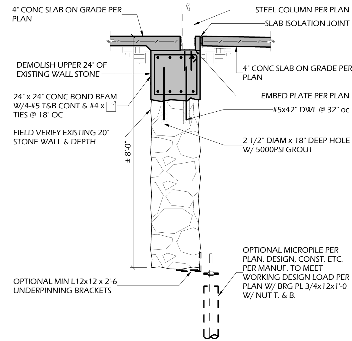
3 SECTION S3.10 1/2' = 1'-0"
