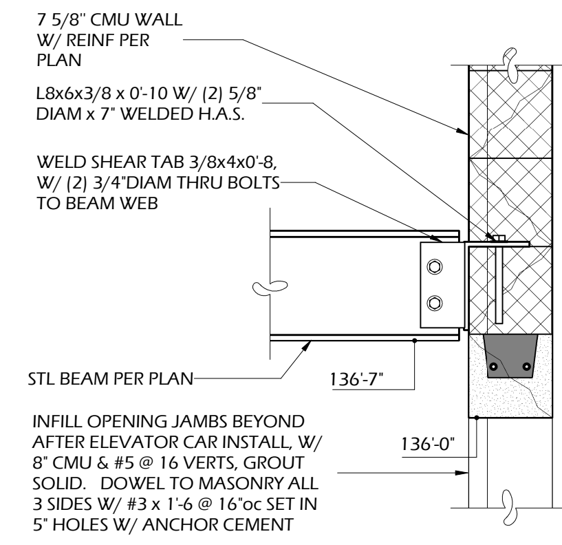
4 SECTION S3.10 1' = 1'-0"
