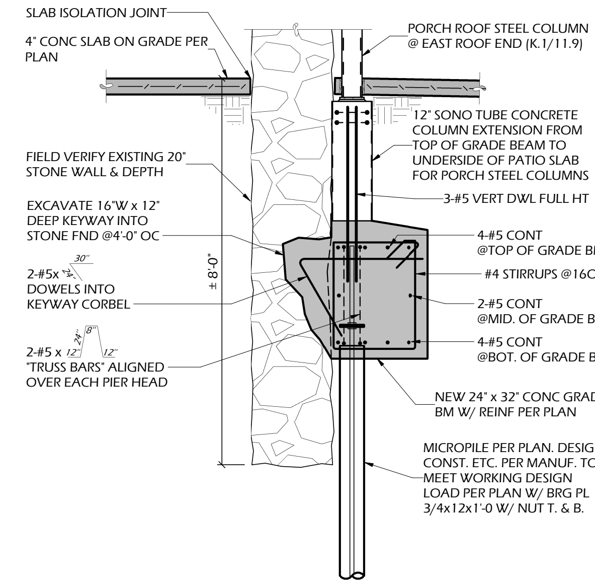
2 SECTION S3.10 1/2' = 1'-0"
