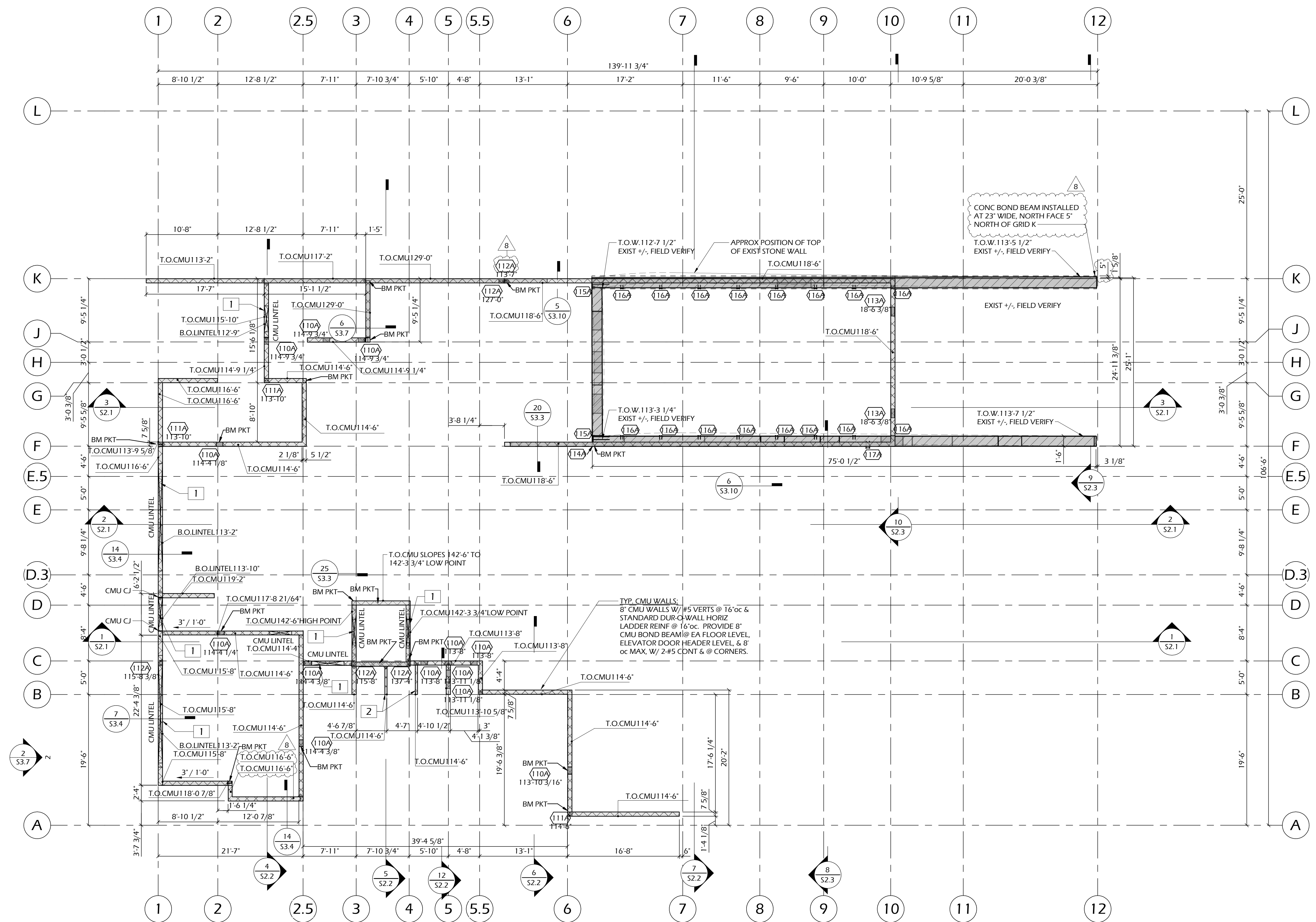
1 PLAN FOR CMU WALLS 1/8" = 1'-0" * ALL CMU WALLS ARE NOMINAL 8" CMU (7 5/8") UNLESS OTHERWISE NOTED
