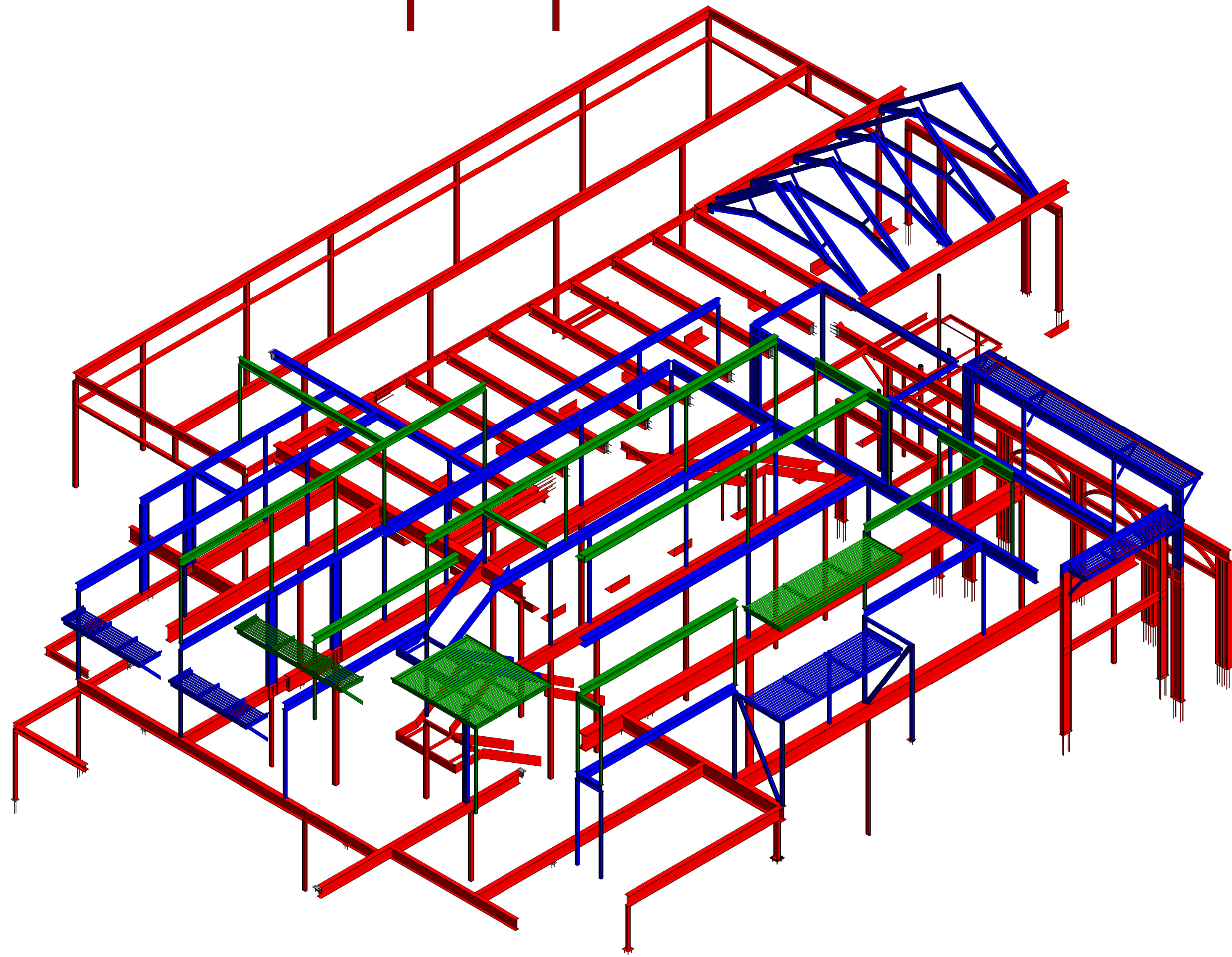
1 S0.5 STRUCTURAL STEEL FRAMING ISOMETRIC VIEW ILLUSTRATIVE / FOR VISUAL REFERENCE PURPOSES ONLY (SOUTHWEST)
